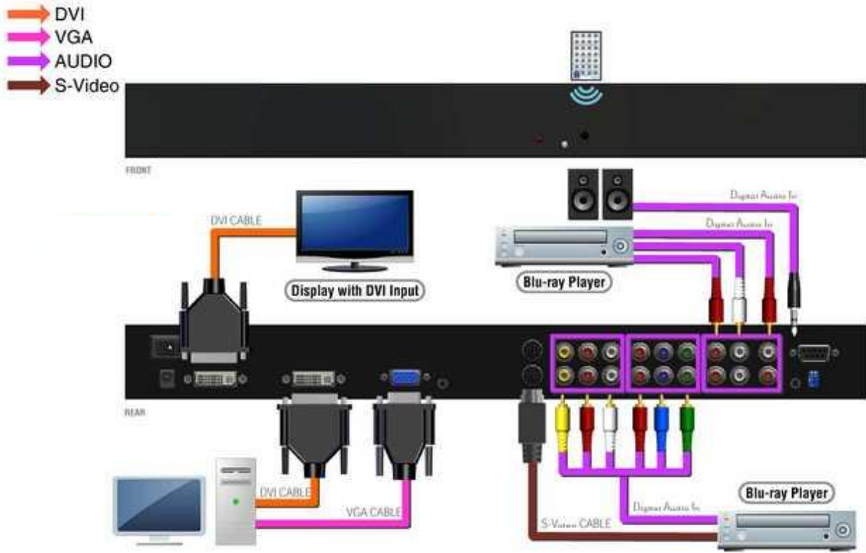
Figure 1: Configuration Diagram
