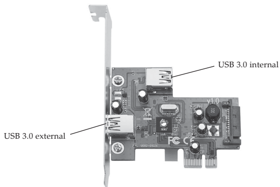
Figure 2: JU-P20512-S1 Layout
