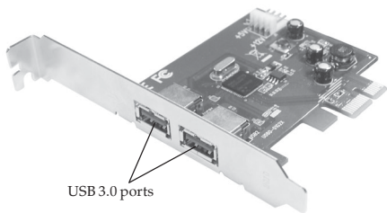
Figure 1: JU-P20412-S2 Layout
